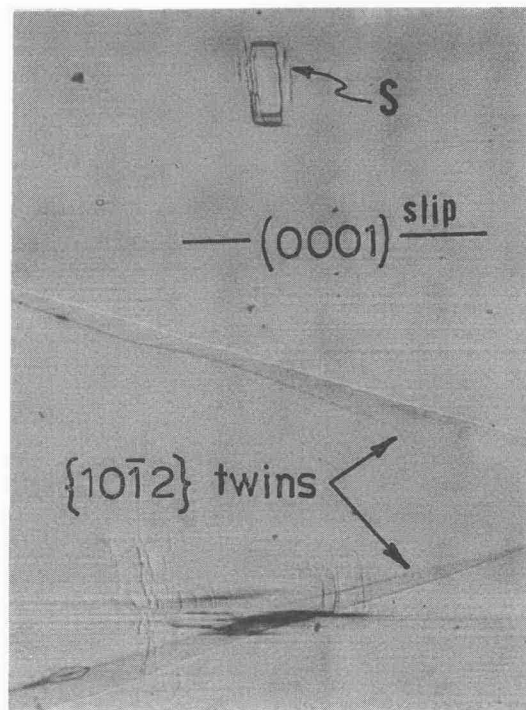
Fig. 3 - Optical Photomicrograph Showing (0001) Slip Lines, \{10\bar{1}2\} Twins and Rectangular Markings at S on (11\bar{2}0) Surface of Crystal ISR-10 Shown in Figure 1. Mag. 240X
